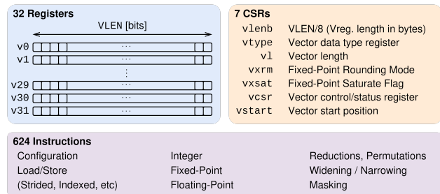
Fig. 1: Overview of the RISC-V "V" Vector Extension (RVV)
